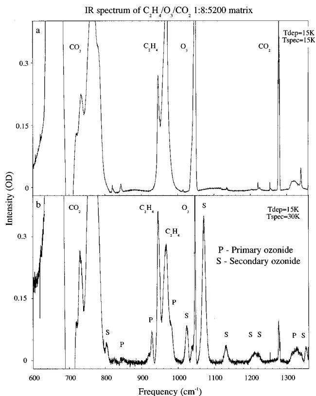
Figure 3. Infrared spectra of solid \text{CO}_2 matrices obtained upon codeposition of ethylene and ozone. (a) The spectrum of a \text{CO}_2 matrix deposited at 15 K, taken at 15 K. (b) The spectrum of the same matrix recorded at 30 K, after being kept at that temperature for 30 min.
