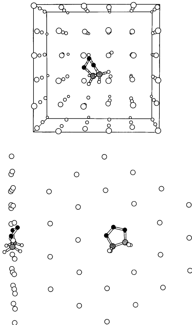
Figure 4. The structure of the most frequently obtained trapping site of POZ deposited in an argon fcc lattice at 25 K as calculated by the molecular dynamics simulation. Only a small portion of the actually calculated structure is shown, to facilitate the exposition of the geometry near the trapped molecule. The molecule is seen to displace three argon atoms from a 111 plane of the crystal lattice, the displaced atoms forming a triangle. The upper part shows a three-dimensional representation of the site. The bottom part shows cuts taken along the lattice planes in which argon atoms were replaced by the molecule. The key is as follows: argon atoms are shown as open large circles, hydrogen atoms as smaller open circles, oxygen atoms are black, and carbon atoms are gray.
